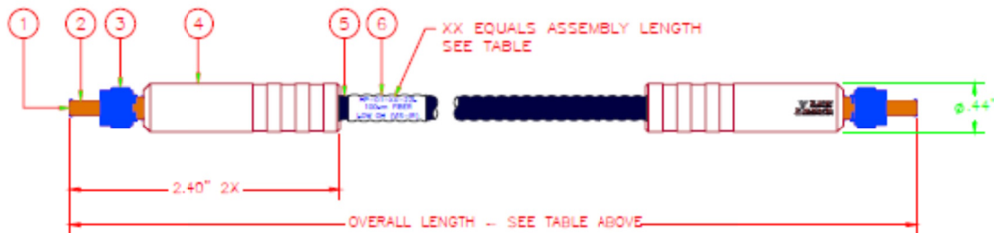
Typical Lee Laser Fiber Optic Cable Delivery Detail.
